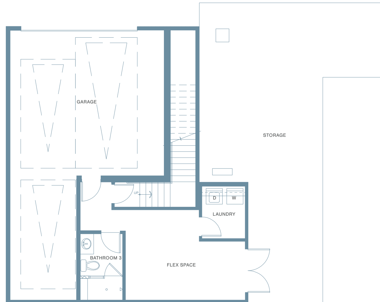
BASEMENT LEVEL
