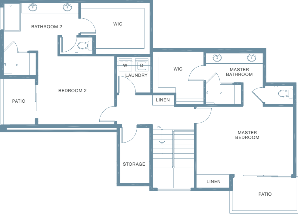
SECOND LEVEL
