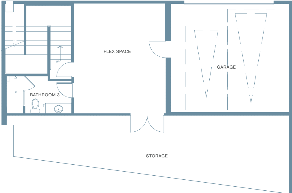
BASEMENT LEVEL
